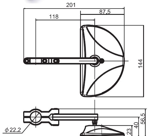
#81001 Handlebar clamp type 1PC
