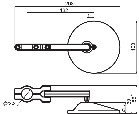
#80917 Handlebar clamp type 1PC
