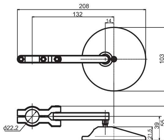
#80917 Handlebar clamp type 1PC
