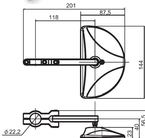
#81001 Handlebar clamp type 1PC
